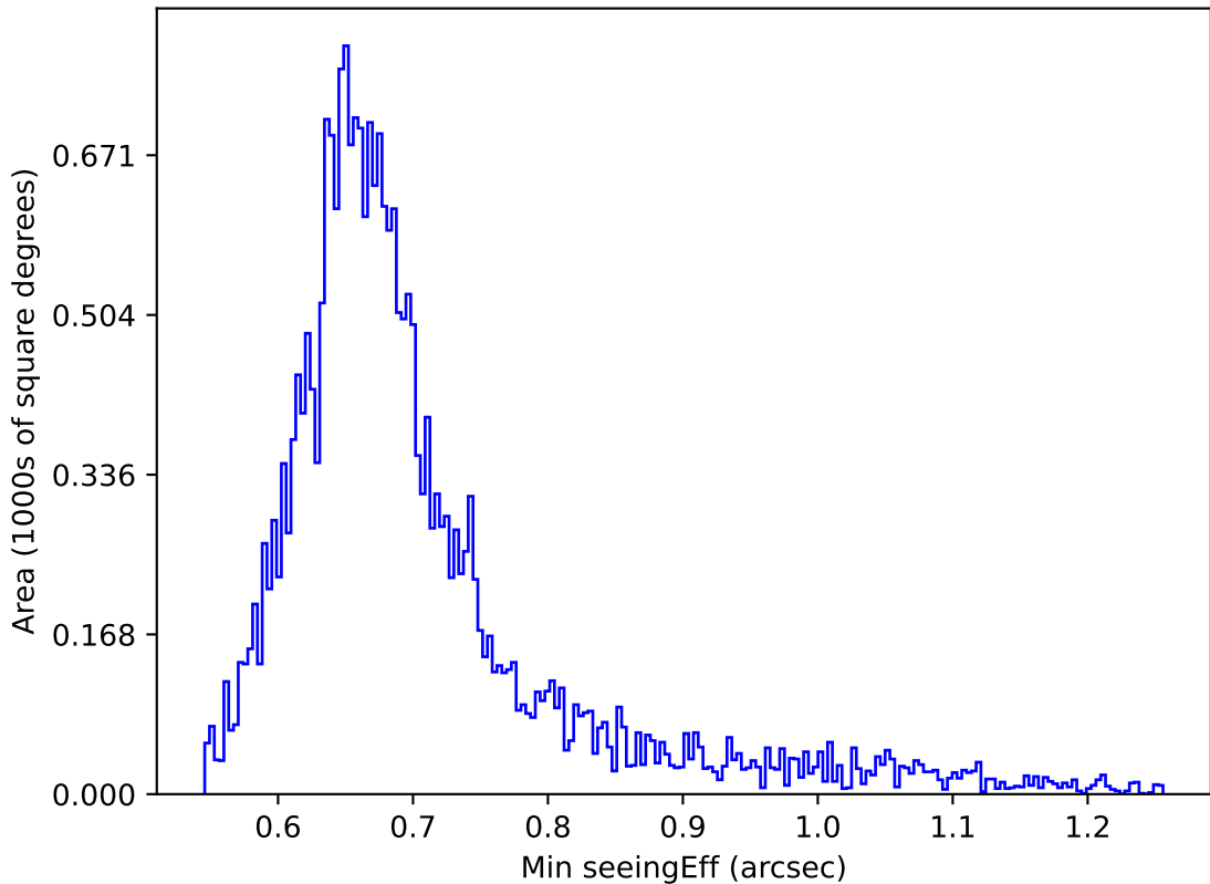
roll_uniform_early_half_mjdp0_v3.4_10yrs Yr 1 i band: Min seeingEff
