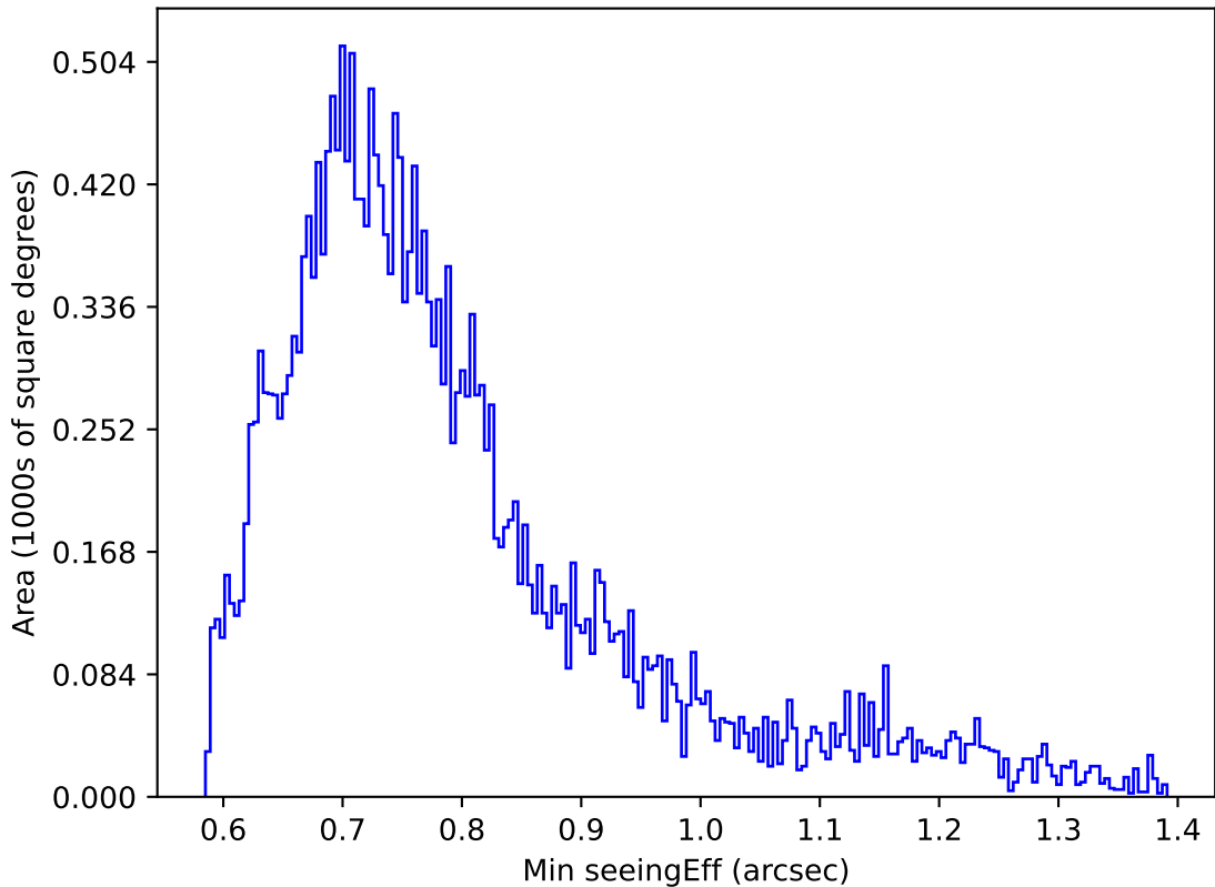
roll_uniform_early_half_mjdp0_v3.4_10yrs Yr 1 g band: Min seeingEff
