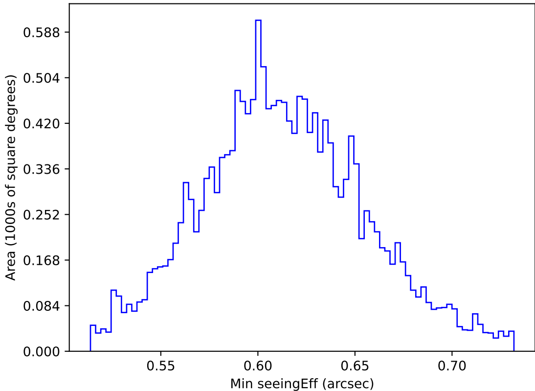
roll_uniform_early_half_mjdp0_v3.4_10yrs WFD z band: Min seeingEff
