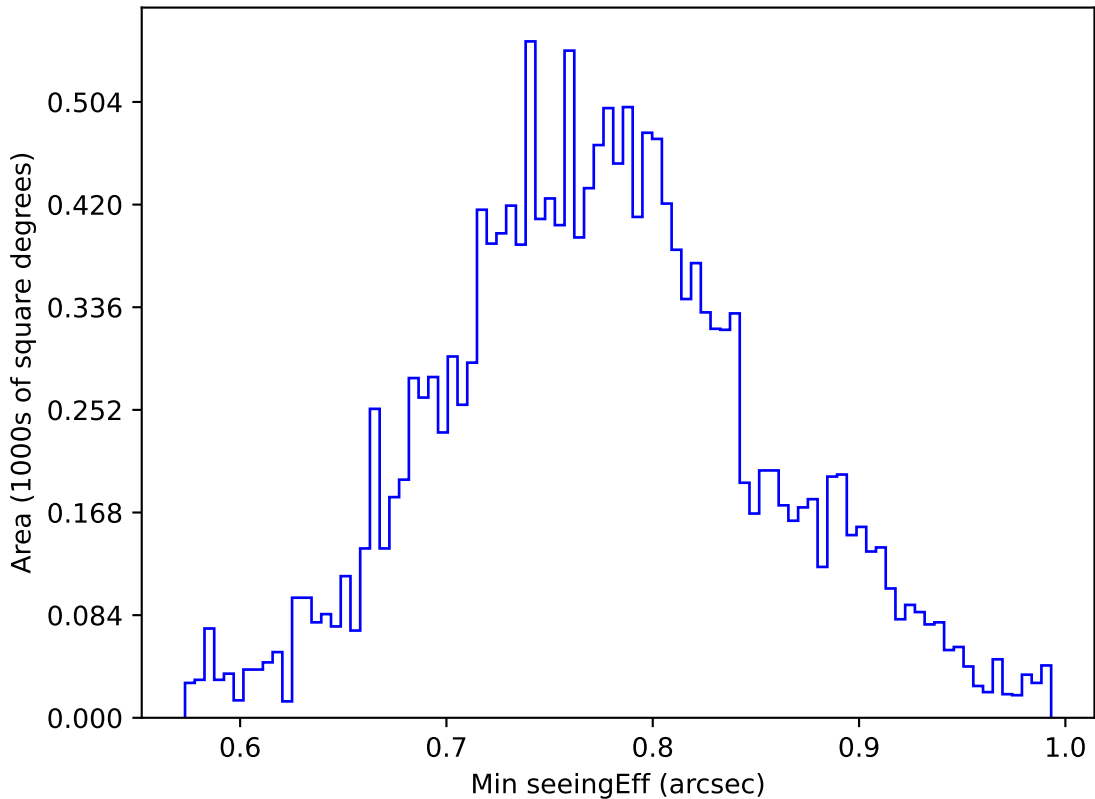
roll_uniform_early_half_mjdp0_v3.4_10yrs WFD u band: Min seeingEff
