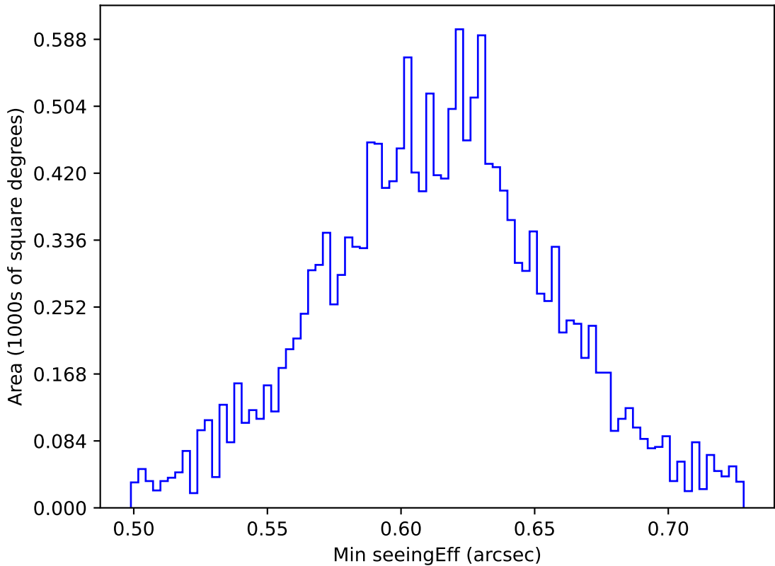
roll_uniform_early_half_mjdp0_v3.4_10yrs WFD r band: Min seeingEff
