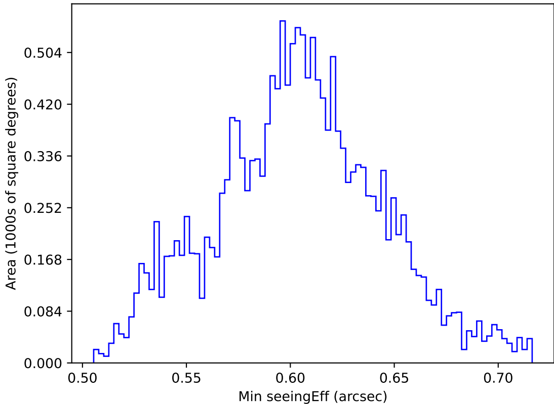
roll_uniform_early_half_mjdp0_v3.4_10yrs WFD i band: Min seeingEff
