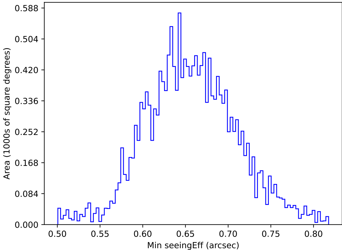
roll_uniform_early_half_mjdp0_v3.4_10yrs WFD g band: Min seeingEff
