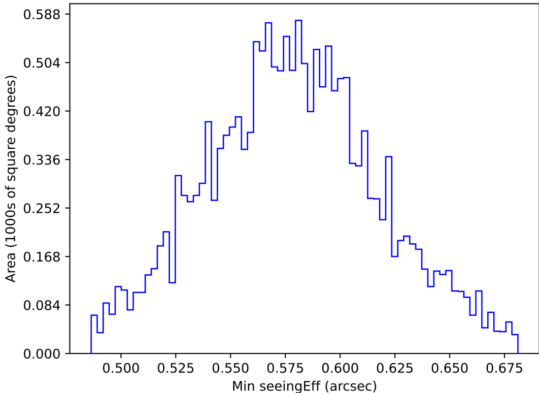
roll_uniform_early_half_mjdp0_v3.4_10yrs WFD all bands: Min seeingEff
