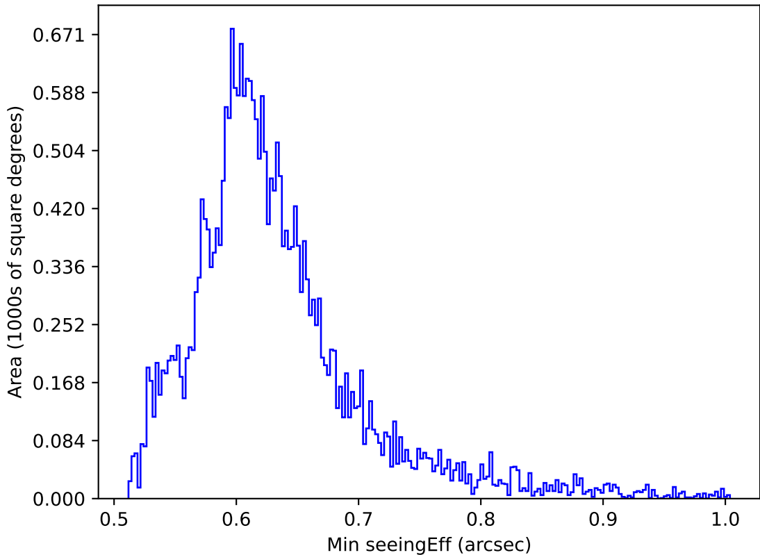
roll_uniform_early_half_mjdp0_v3.4_10yrs All sky i band: Min seeingEff
