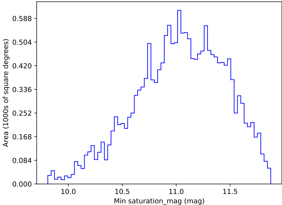
roll_uniform_early_half_mjdp0_v3.4_10yrs WFD all bands: Min saturation_mag
