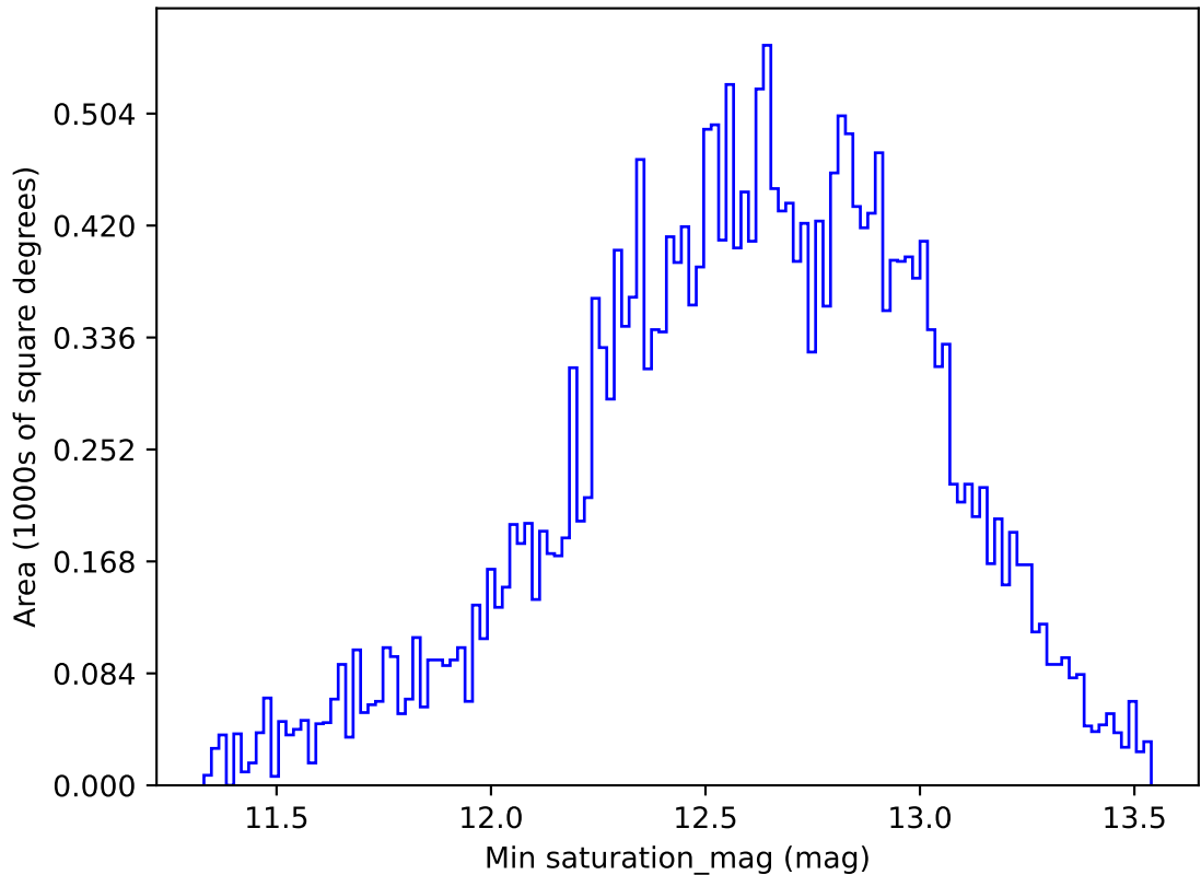
roll_uniform_early_half_mjdp0_v3.4_10yrs All sky r band: Min saturation_mag
