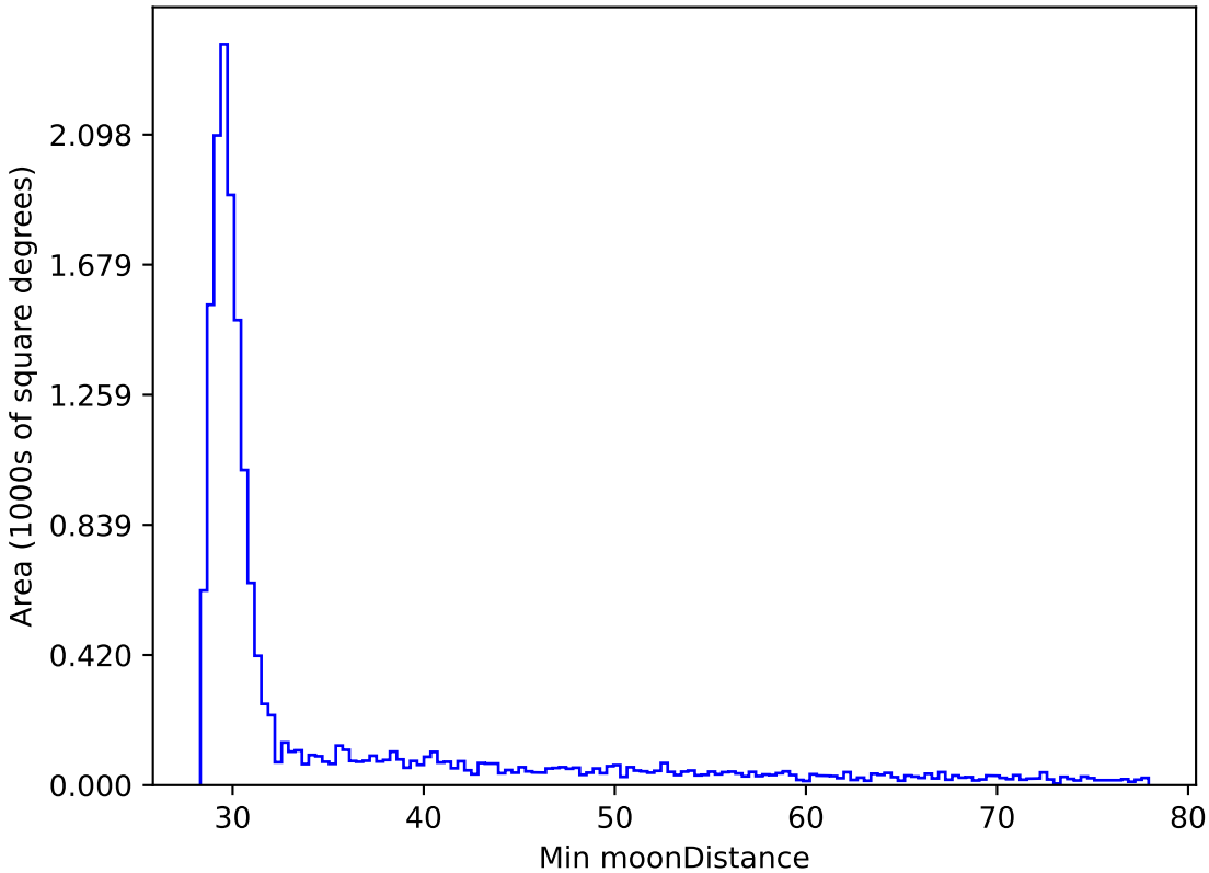
roll_uniform_early_half_mjdp0_v3.4_10yrs WFD z band: Min moonDistance
