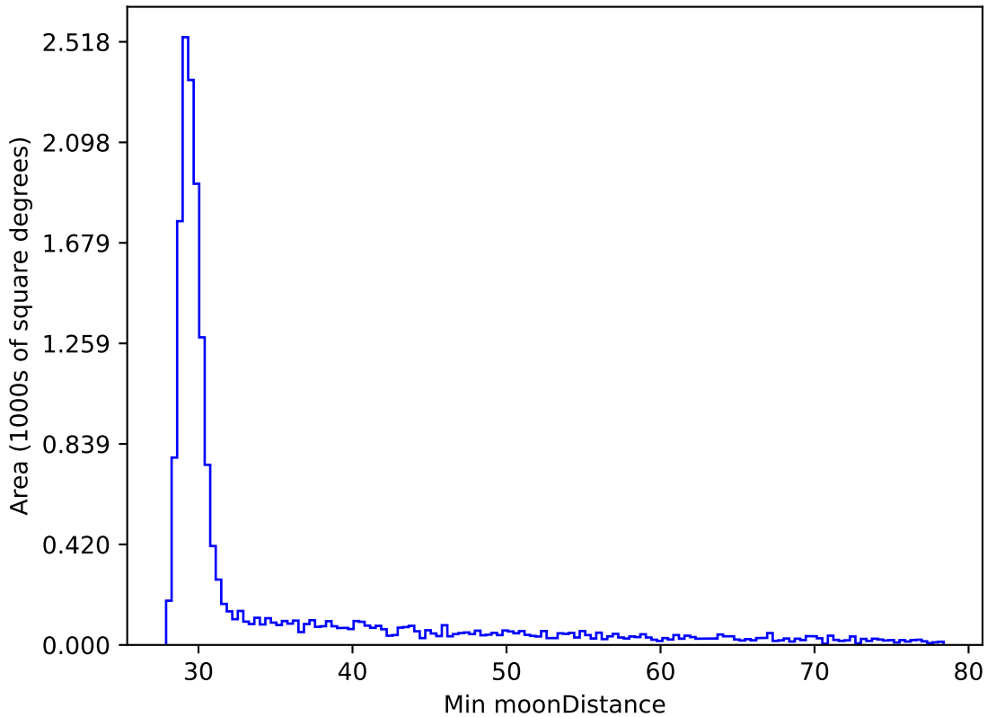
roll_uniform_early_half_mjdp0_v3.4_10yrs WFD y band: Min moonDistance
