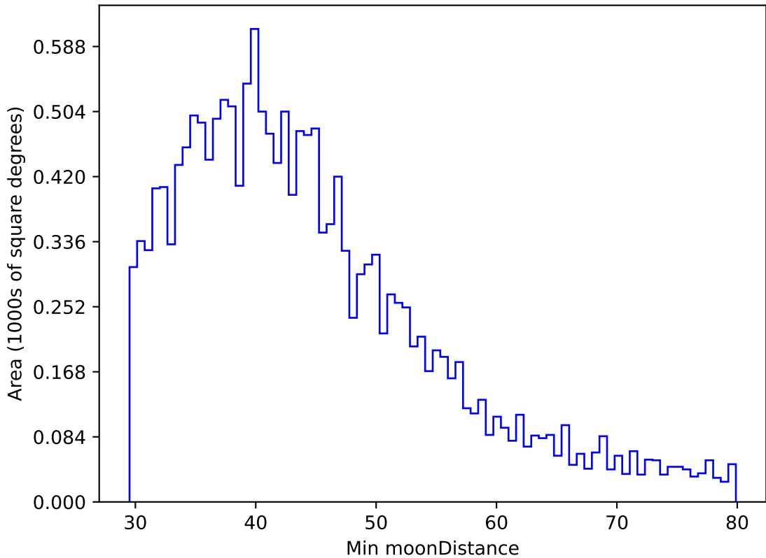
roll_uniform_early_half_mjdp0_v3.4_10yrs WFD g band: Min moonDistance
