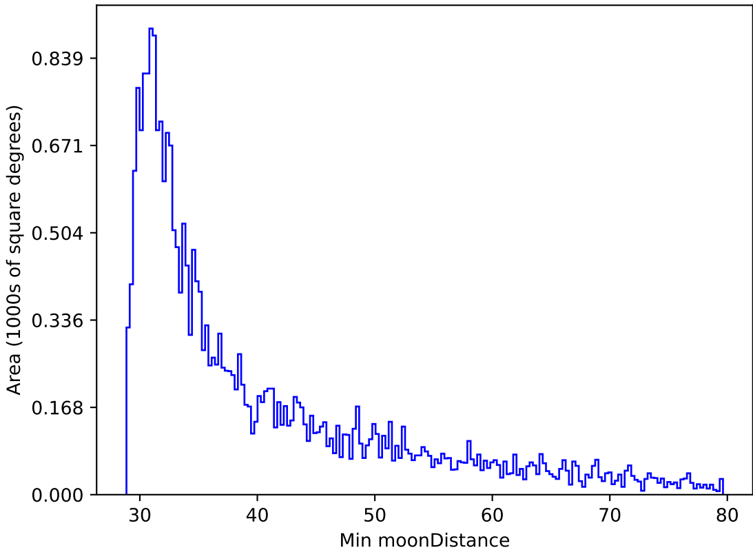
roll_uniform_early_half_mjdp0_v3.4_10yrs All sky r band: Min moonDistance
