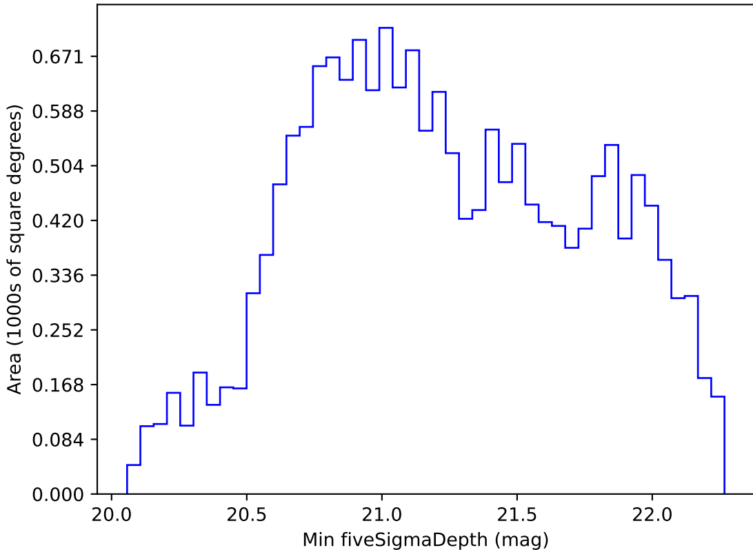
roll_uniform_early_half_mjdp0_v3.4_10yrs WFD z band: Min fiveSigmaDepth
