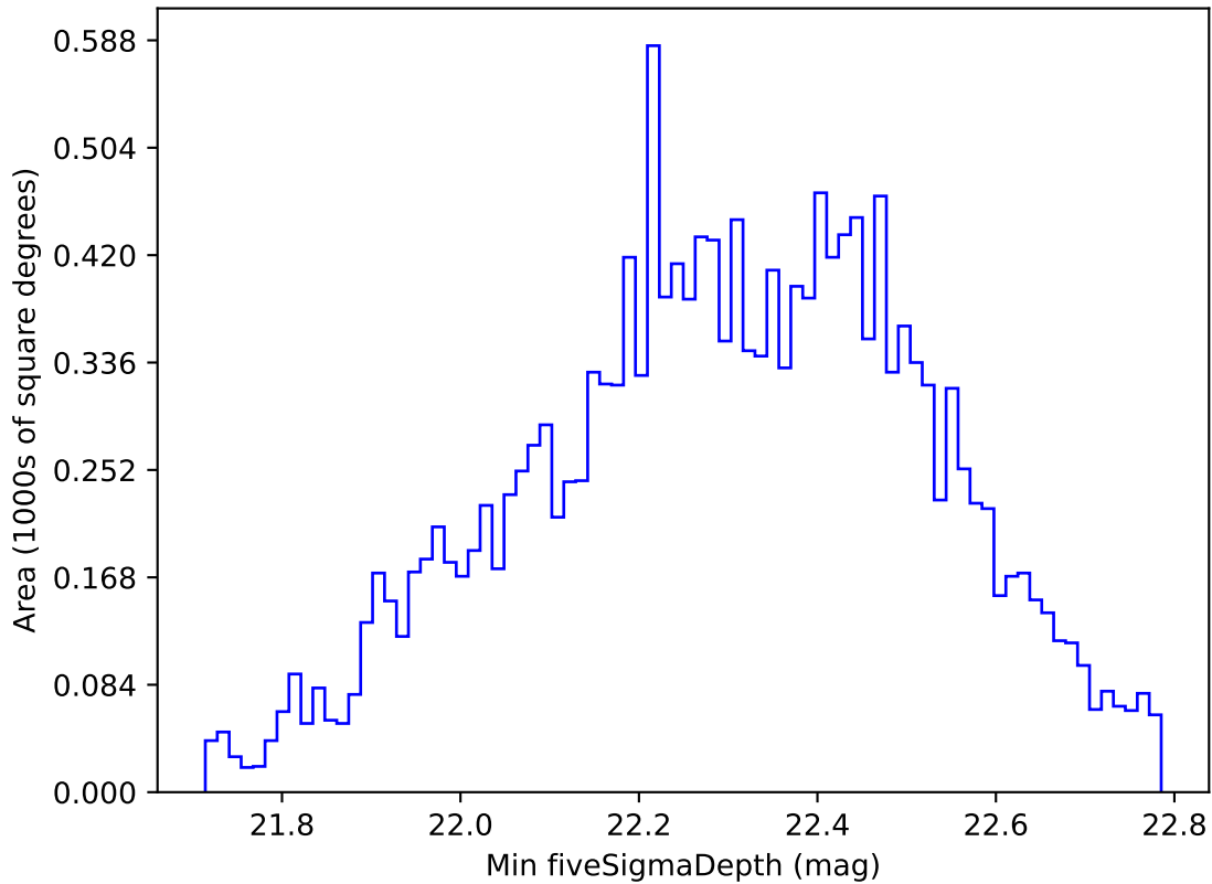
roll_uniform_early_half_mjdp0_v3.4_10yrs WFD u band: Min fiveSigmaDepth
