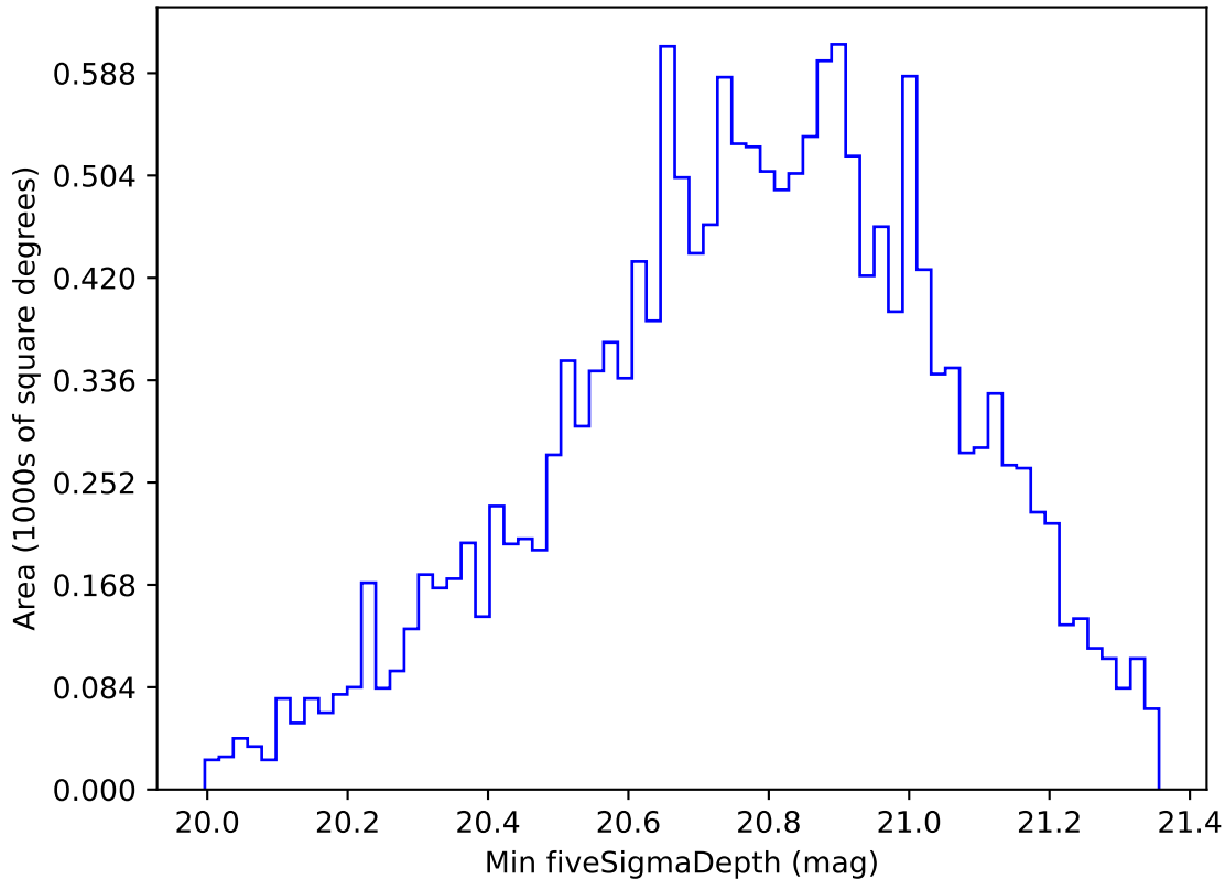
roll_uniform_early_half_mjdp0_v3.4_10yrs WFD all bands: Min fiveSigmaDepth
