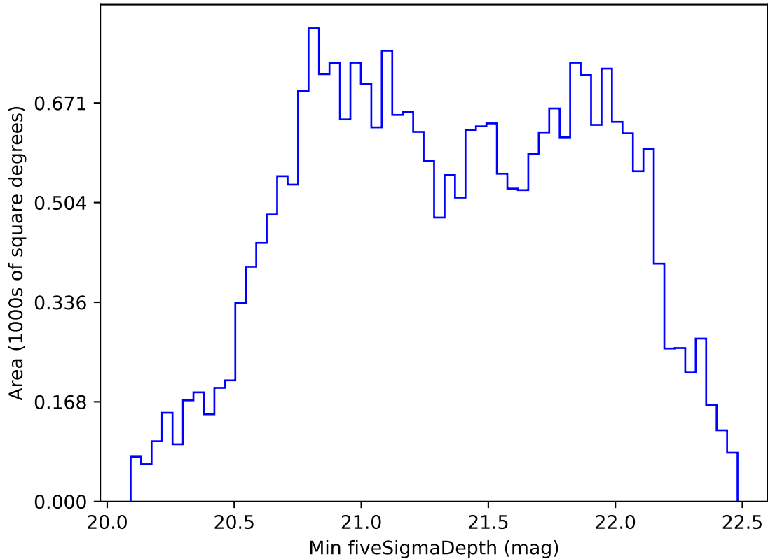
roll_uniform_early_half_mjdp0_v3.4_10yrs All sky z band: Min fiveSigmaDepth
