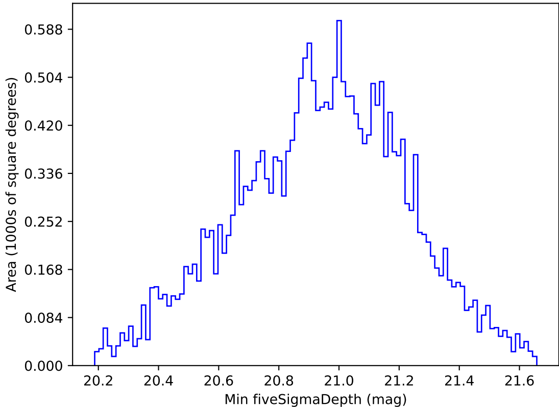
roll_uniform_early_half_mjdp0_v3.4_10yrs All sky y band: Min fiveSigmaDepth
