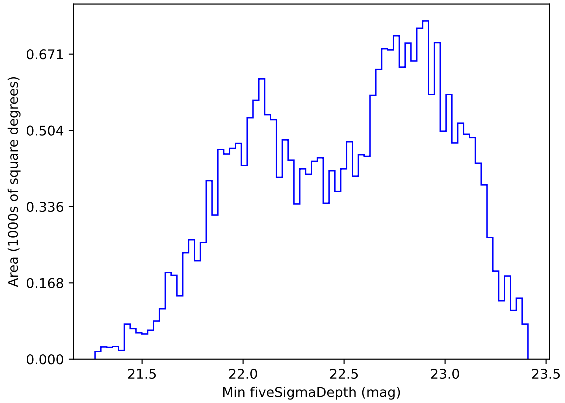
roll_uniform_early_half_mjdp0_v3.4_10yrs All sky r band: Min fiveSigmaDepth
