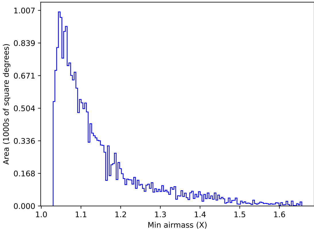
roll_uniform_early_half_mjdp0_v3.4_10yrs Yr 1 u band: Min airmass
