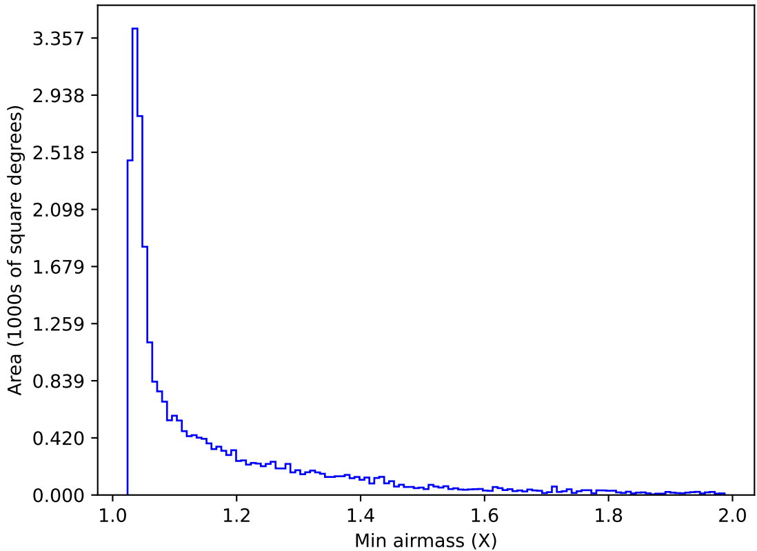
roll_uniform_early_half_mjdp0_v3.4_10yrs Yr 1 r band: Min airmass
