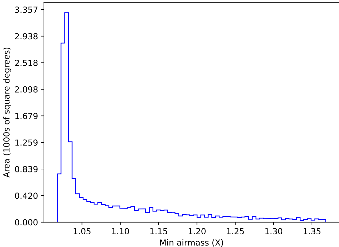
roll_uniform_early_half_mjdp0_v3.4_10yrs WFD z band: Min airmass
