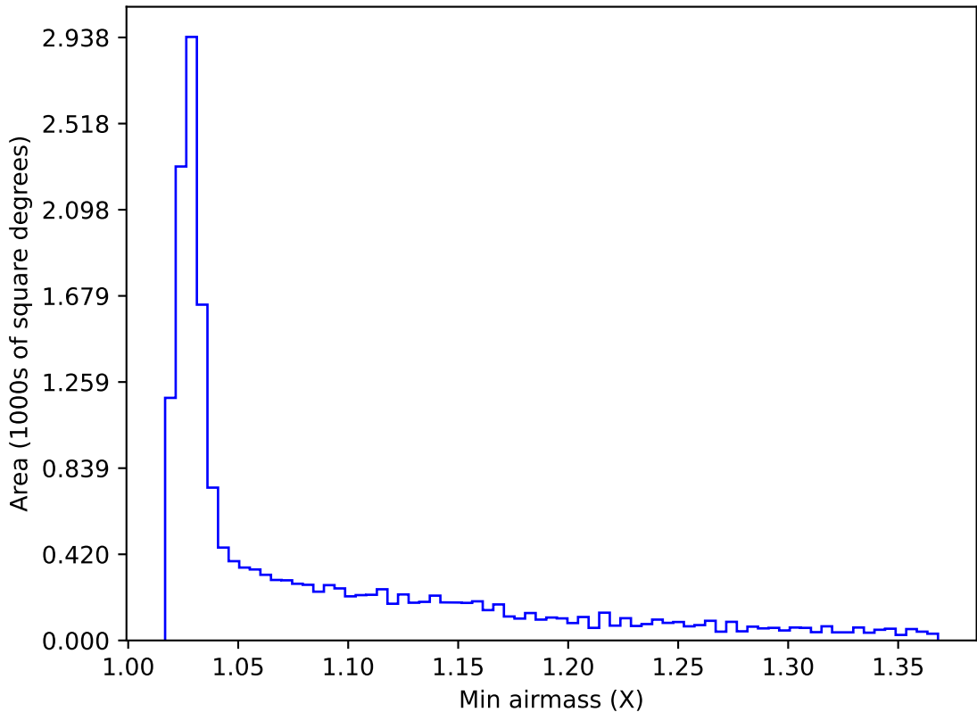
roll_uniform_early_half_mjdp0_v3.4_10yrs WFD r band: Min airmass
