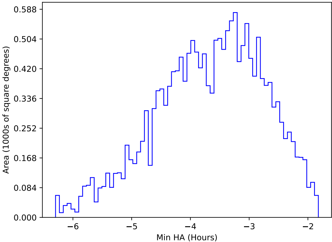
roll_uniform_early_half_mjdp0_v3.4_10yrs WFD y band: Min HA
