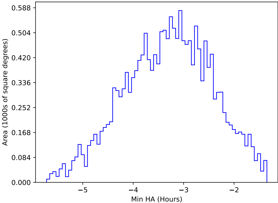
roll_uniform_early_half_mjdp0_v3.4_10yrs WFD u band: Min HA
