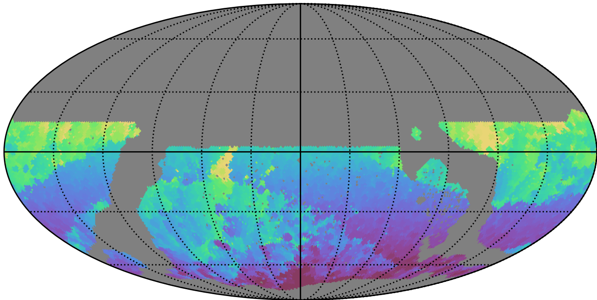
roll_uniform_early_half_mjdp0_v3.4_10yrs WFD r band: Min HA
