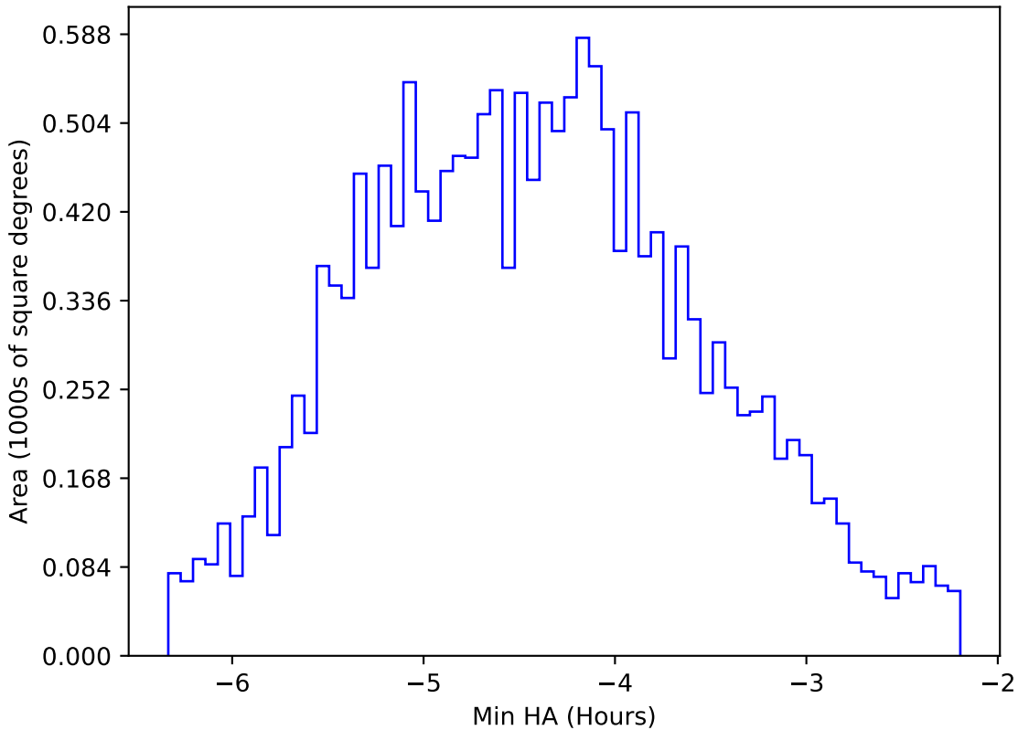
roll_uniform_early_half_mjdp0_v3.4_10yrs WFD r band: Min HA
