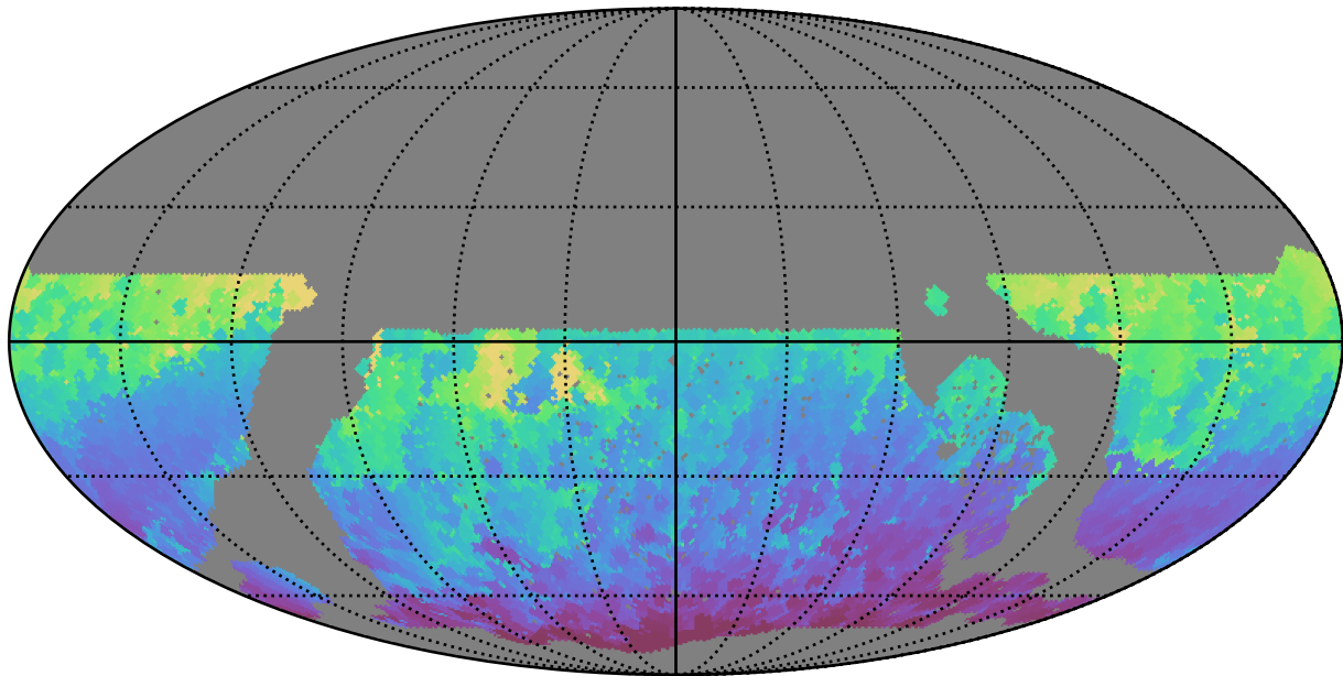
roll_uniform_early_half_mjdp0_v3.4_10yrs WFD i band: Min HA
