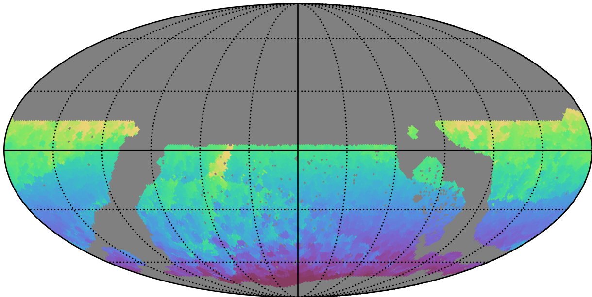
roll_uniform_early_half_mjdp0_v3.4_10yrs WFD all bands: Min HA
