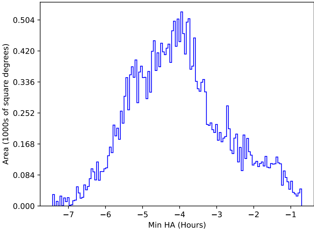
roll_uniform_early_half_mjdp0_v3.4_10yrs All sky z band: Min HA
