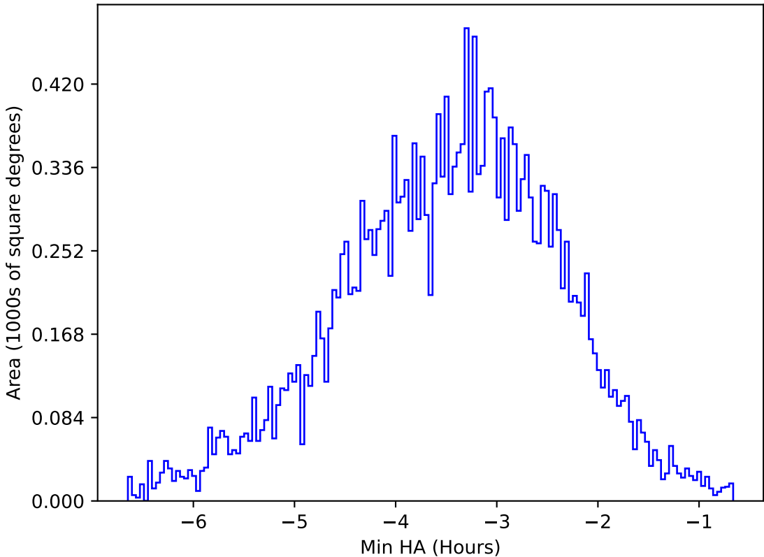
roll_uniform_early_half_mjdp0_v3.4_10yrs All sky y band: Min HA
