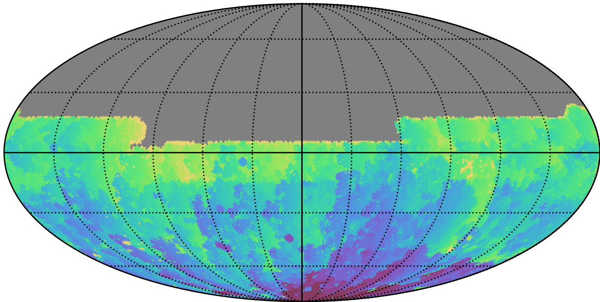
roll_uniform_early_half_mjdp0_v3.4_10yrs All sky u band: Min HA
