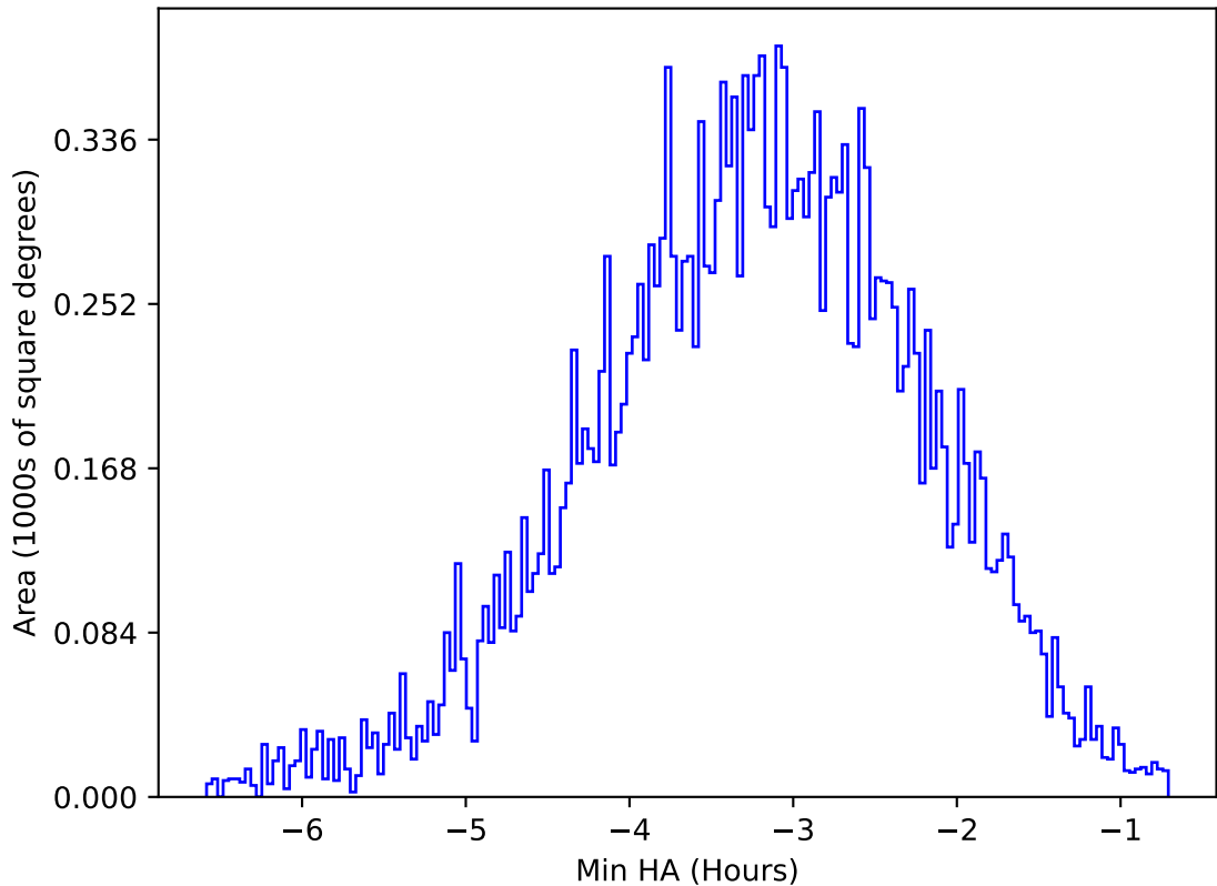
roll_uniform_early_half_mjdp0_v3.4_10yrs All sky u band: Min HA
