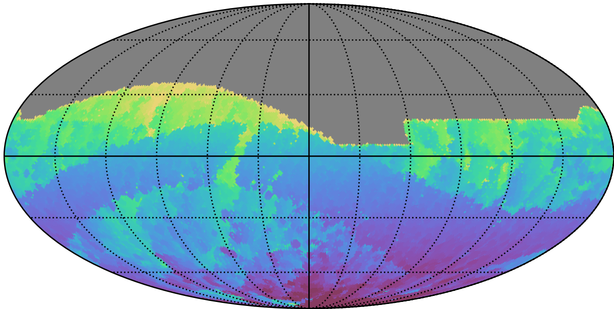
roll_uniform_early_half_mjdp0_v3.4_10yrs All sky r band: Min HA
