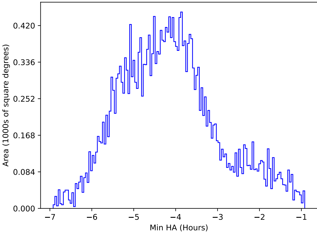
roll_uniform_early_half_mjdp0_v3.4_10yrs All sky r band: Min HA
