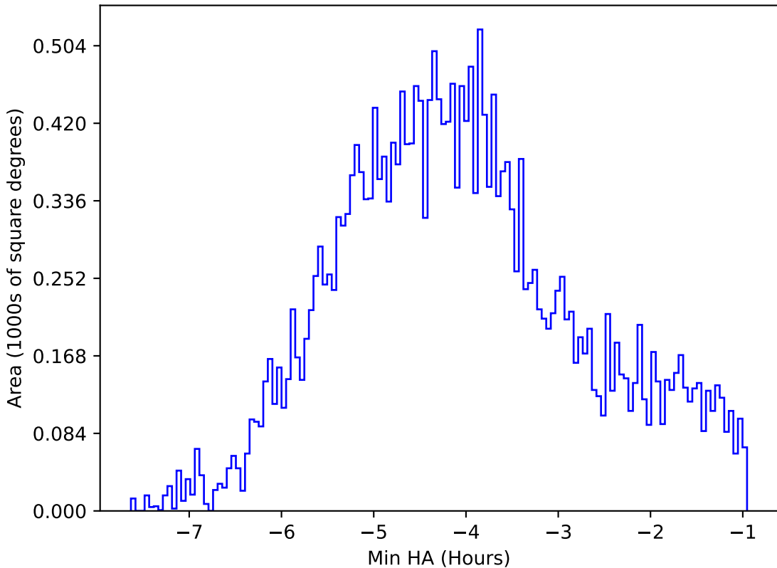
roll_uniform_early_half_mjdp0_v3.4_10yrs All sky i band: Min HA
