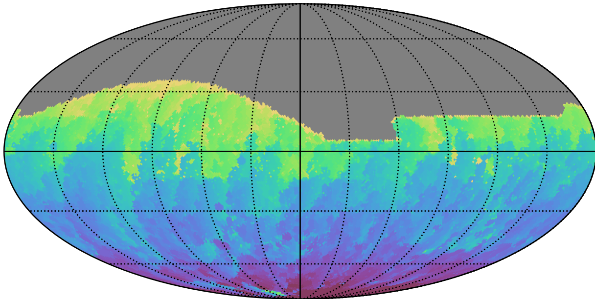
roll_uniform_early_half_mjdp0_v3.4_10yrs All sky g band: Min HA
