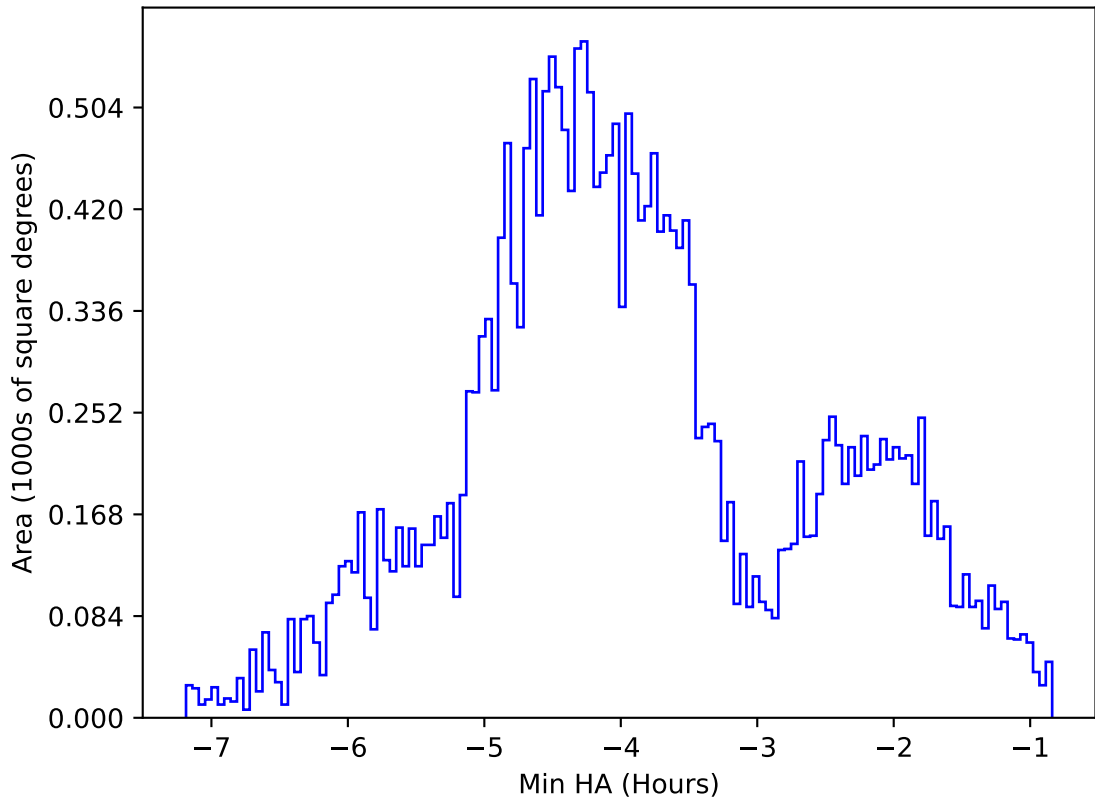
roll_uniform_early_half_mjdp0_v3.4_10yrs All sky g band: Min HA
