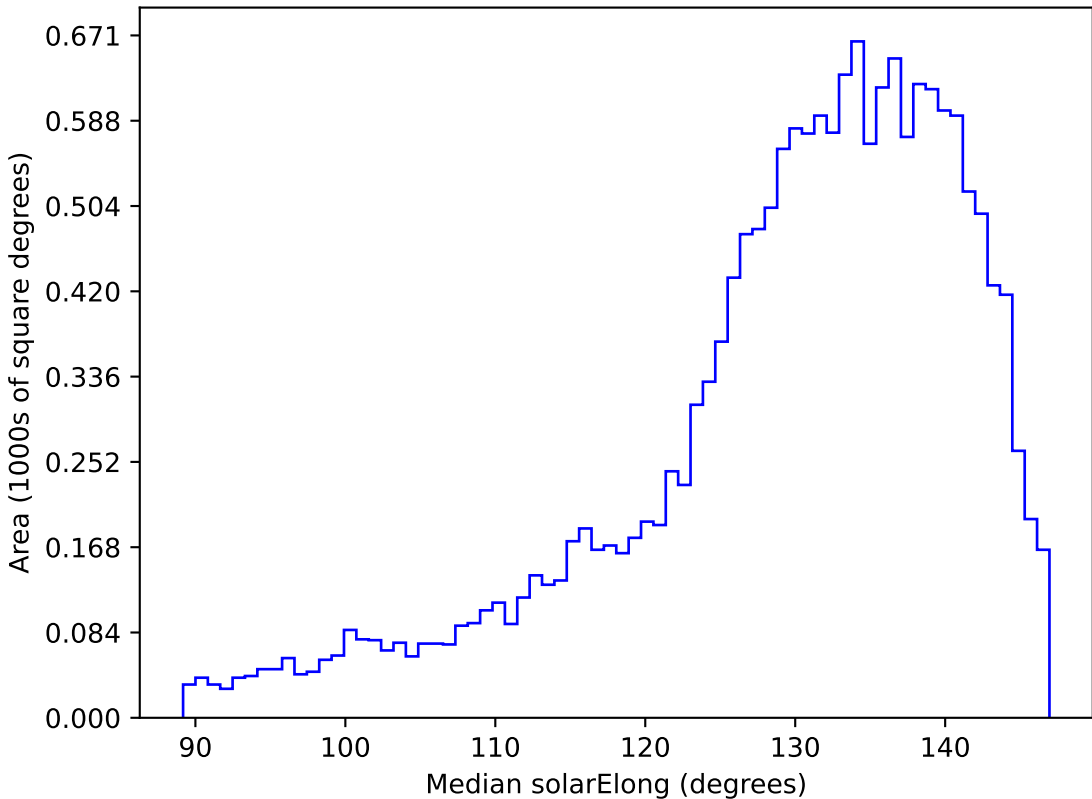
roll_uniform_early_half_mjdp0_v3.4_10yrs WFD y band: Median solarElong
