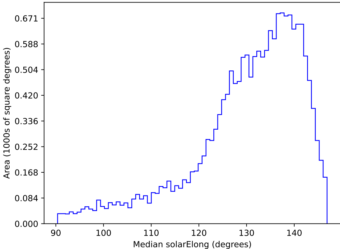
roll_uniform_early_half_mjdp0_v3.4_10yrs WFD r band: Median solarElong
