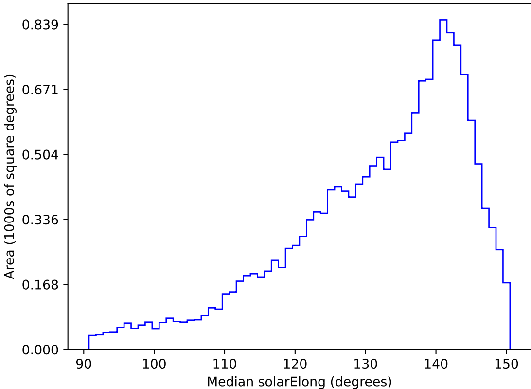
roll_uniform_early_half_mjdp0_v3.4_10yrs WFD g band: Median solarElong
