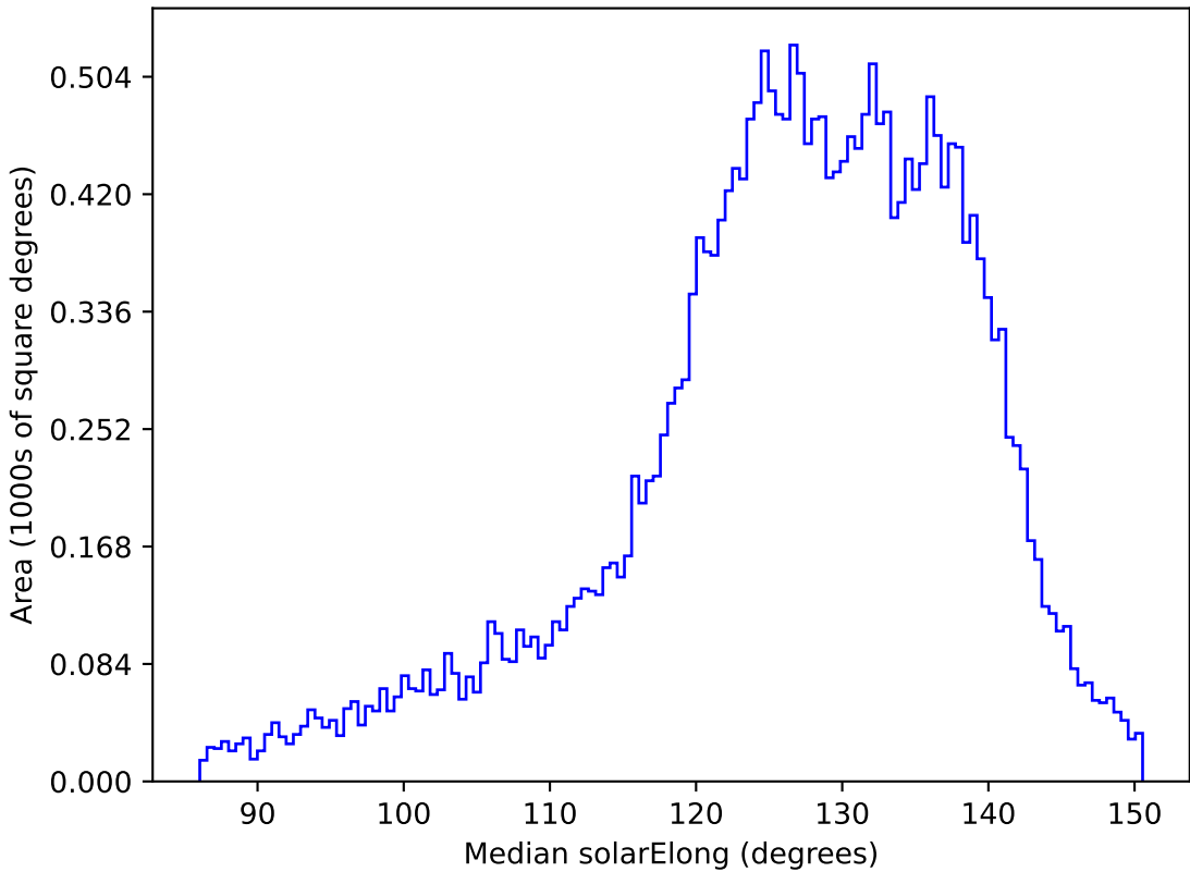
roll_uniform_early_half_mjdp0_v3.4_10yrs All sky z band: Median solarElong
