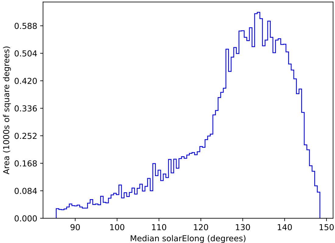
roll_uniform_early_half_mjdp0_v3.4_10yrs All sky y band: Median solarElong
