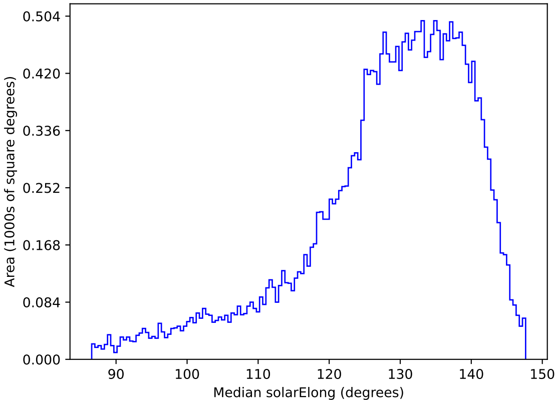
roll_uniform_early_half_mjdp0_v3.4_10yrs All sky i band: Median solarElong
