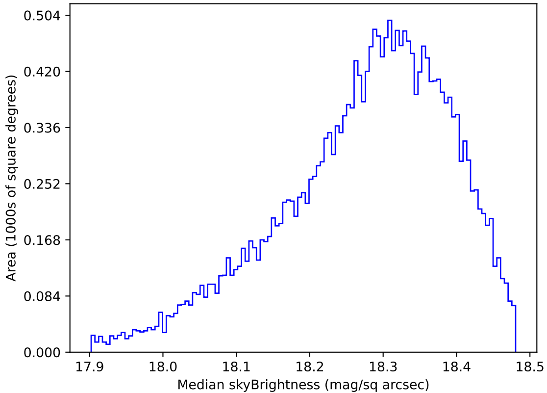
roll_uniform_early_half_mjdp0_v3.4_10yrs Yr 1 y band: Median skyBrightness
