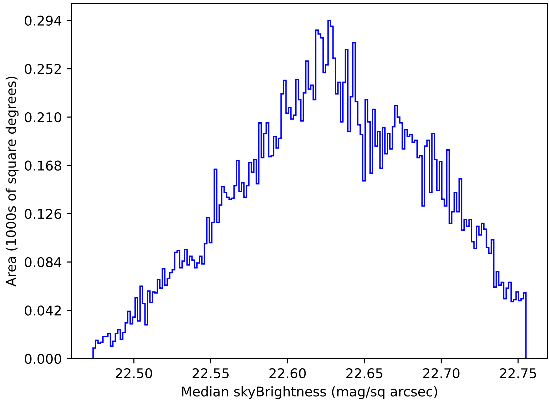
roll_uniform_early_half_mjdp0_v3.4_10yrs Yr 1 u band: Median skyBrightness
