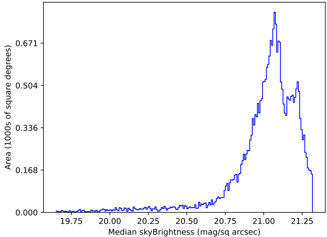
roll_uniform_early_half_mjdp0_v3.4_10yrs Yr 1 r band: Median skyBrightness
