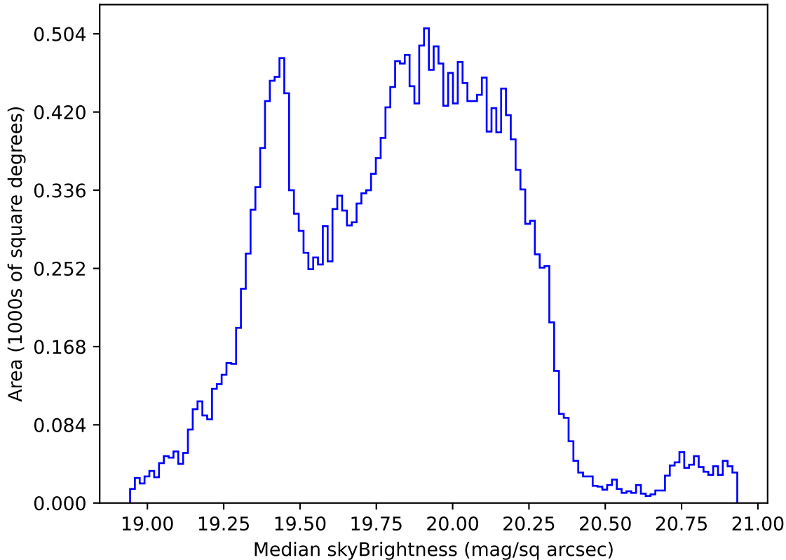
roll_uniform_early_half_mjdp0_v3.4_10yrs Yr 1 all bands: Median skyBrightness
